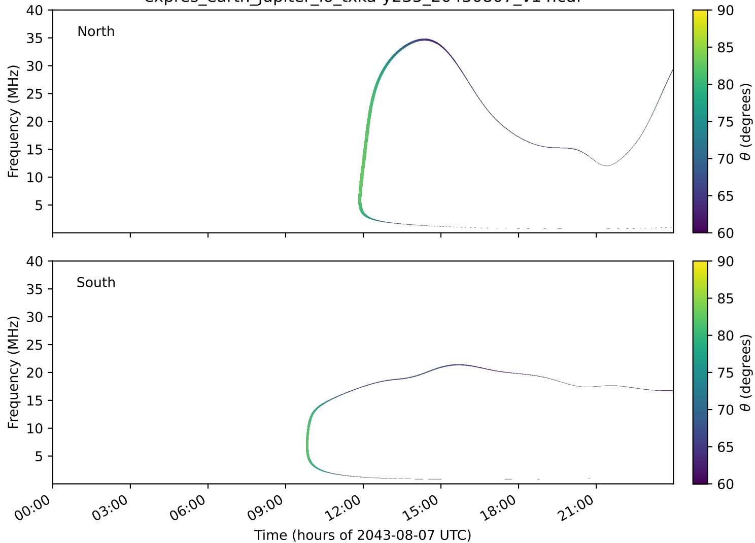
expres_earth_jupiter_io_txka-y235_20430807_v14.cdf
