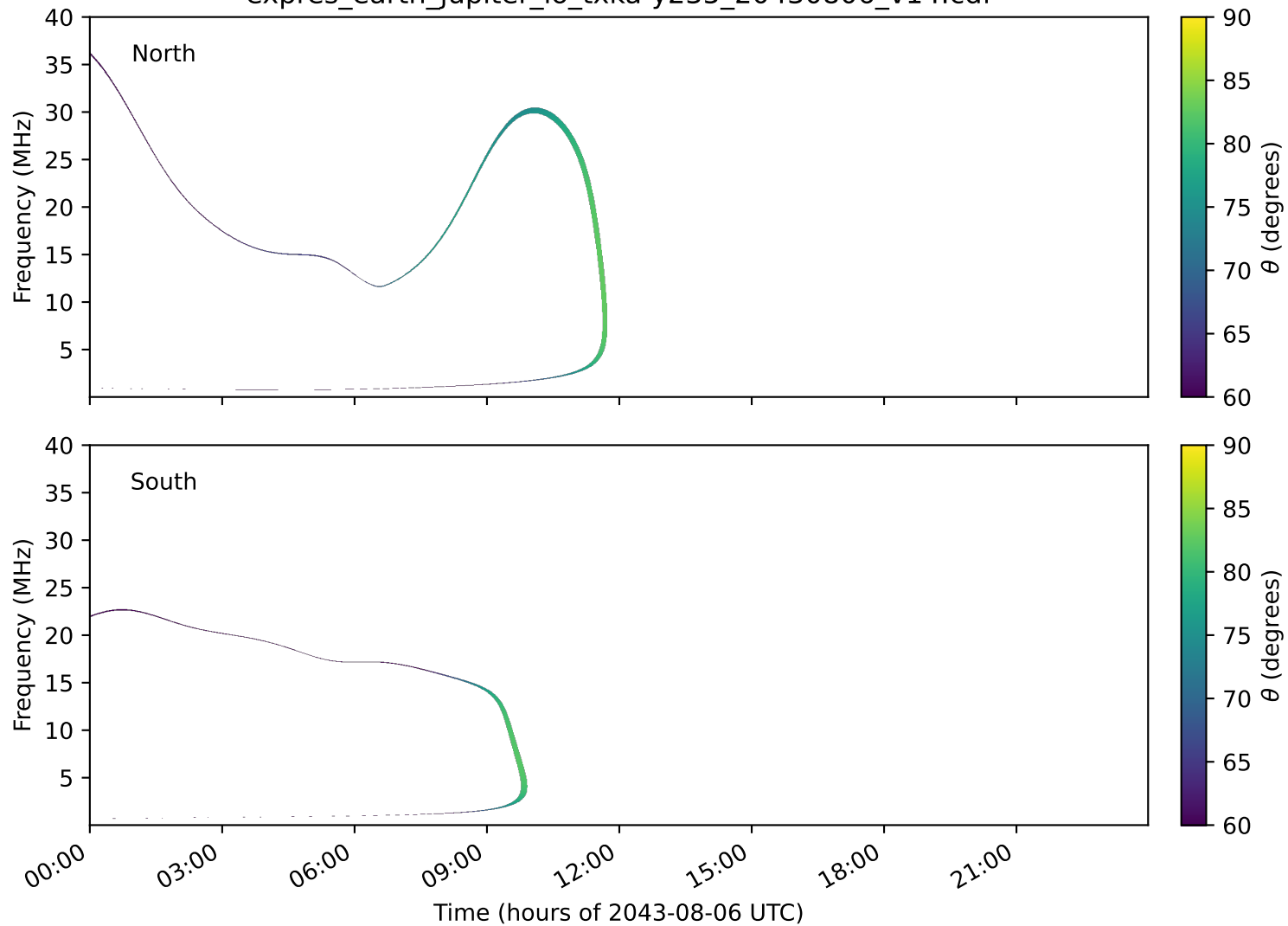
expres_earth_jupiter_io_txka-y235_20430806_v14.cdf
