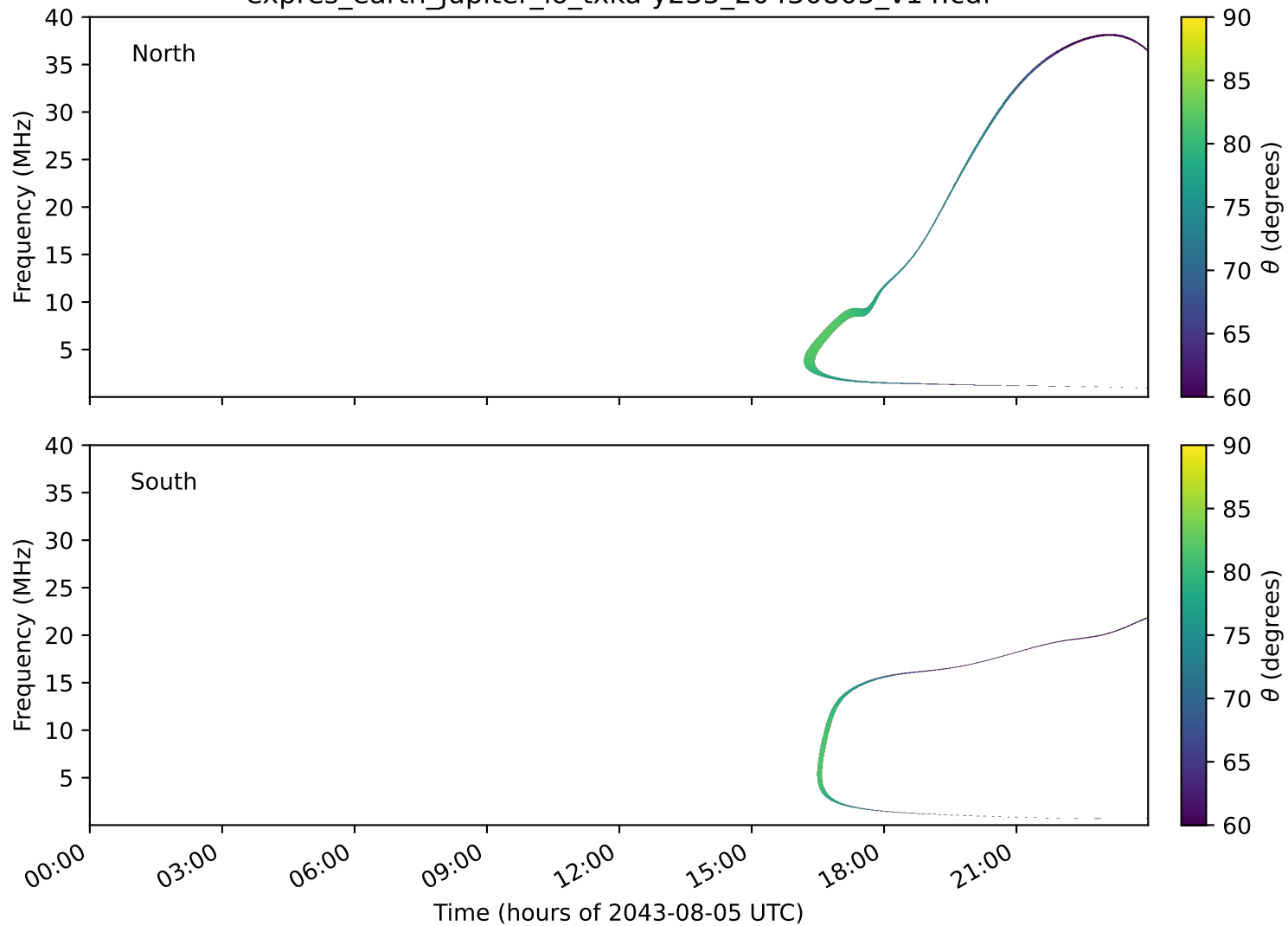
expres_earth_jupiter_io_txka-y235_20430805_v14.cdf
