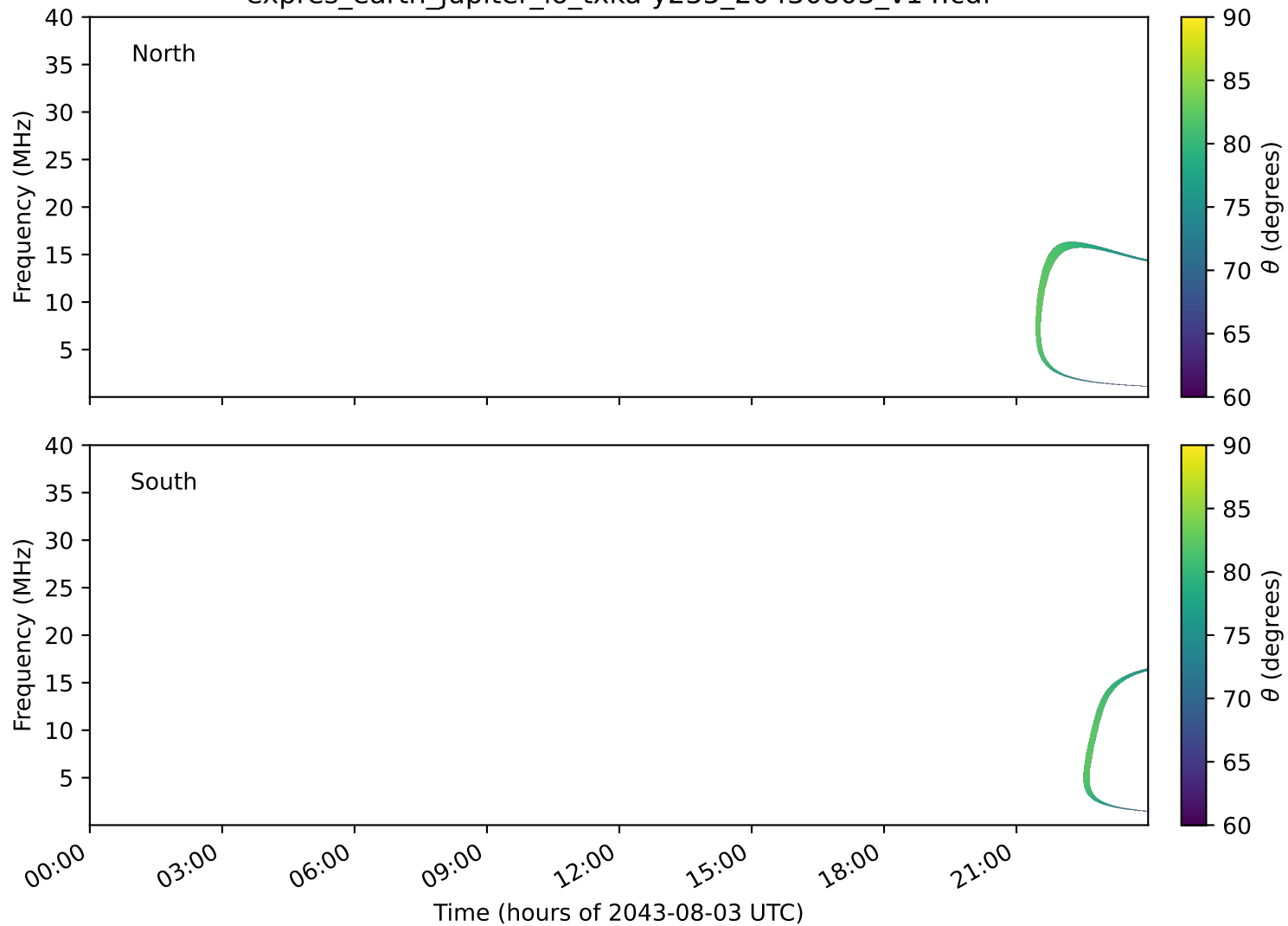
expres_earth_jupiter_io_txka-y235_20430803_v14.cdf
