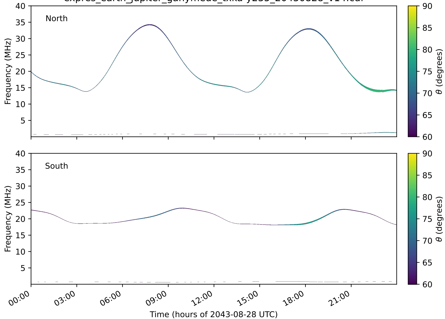
expres_earth_jupiter_ganymede_txka-y235_20430828_v14.cdf
