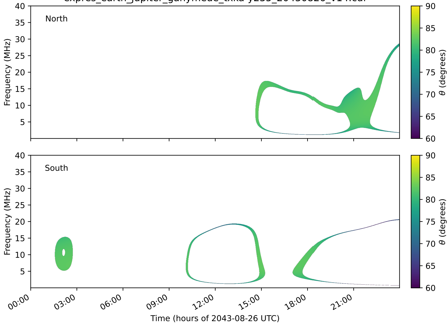
expres_earth_jupiter_ganymede_txka-y235_20430826_v14.cdf
