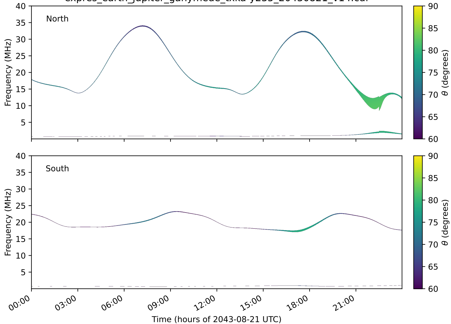
expres_earth_jupiter_ganymede_txka-y235_20430821_v14.cdf
