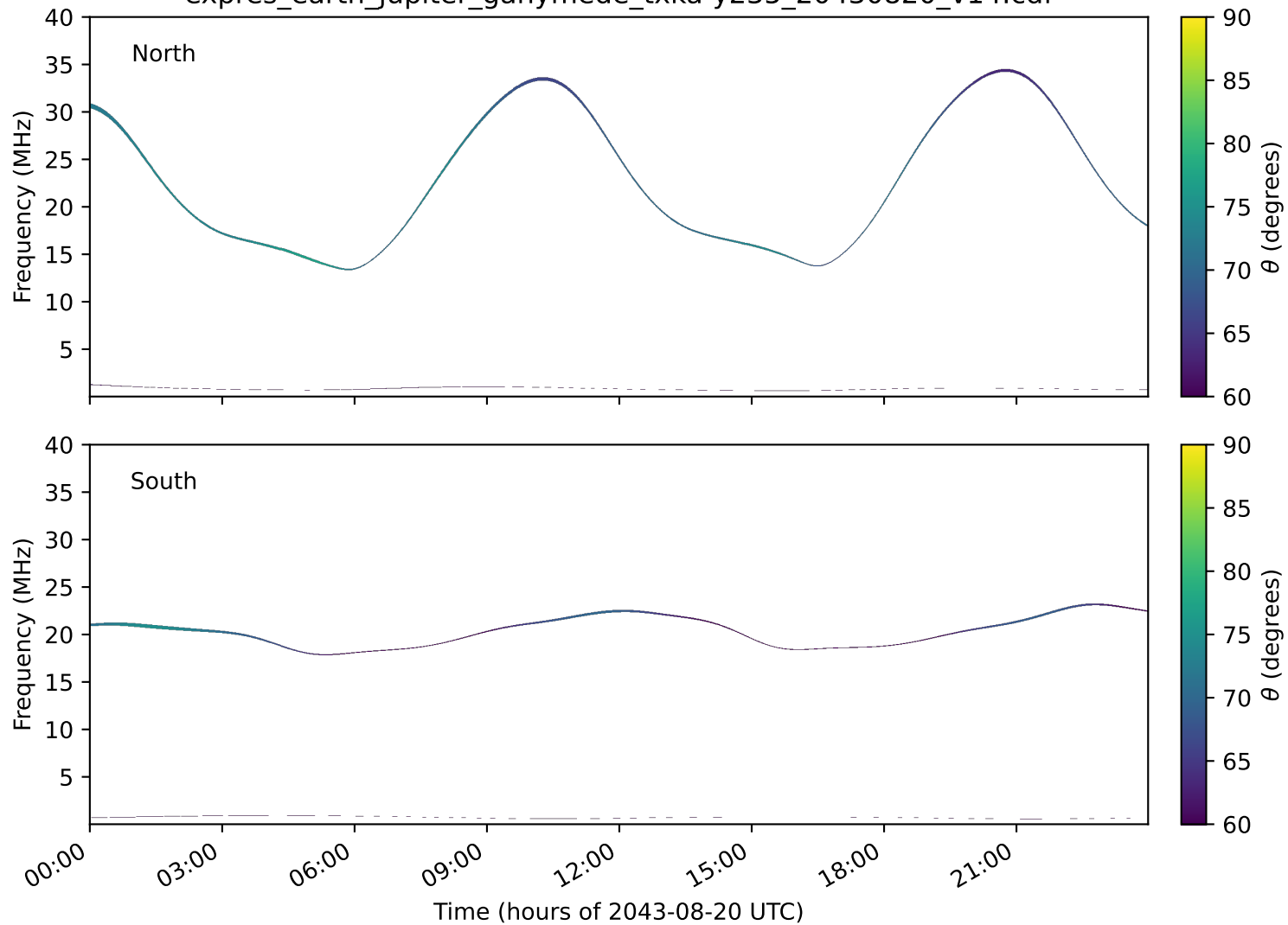
expres_earth_jupiter_ganymede_txka-y235_20430820_v14.cdf
