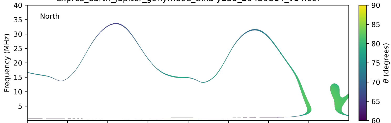
expres_earth_jupiter_ganymede_txka-y235_20430814_v14.cdf
