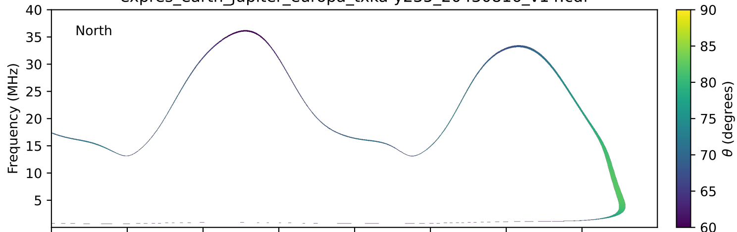
expres_earth_jupiter_europa_txka-y235_20430816_v14.cdf
