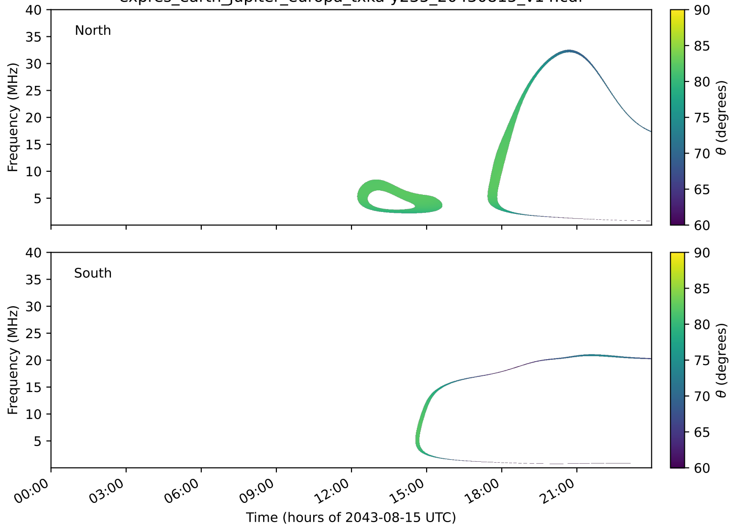
expres_earth_jupiter_europa_txka-y235_20430815_v14.cdf
