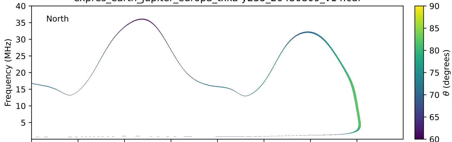
expres_earth_jupiter_europa_txka-y235_20430809_v14.cdf
