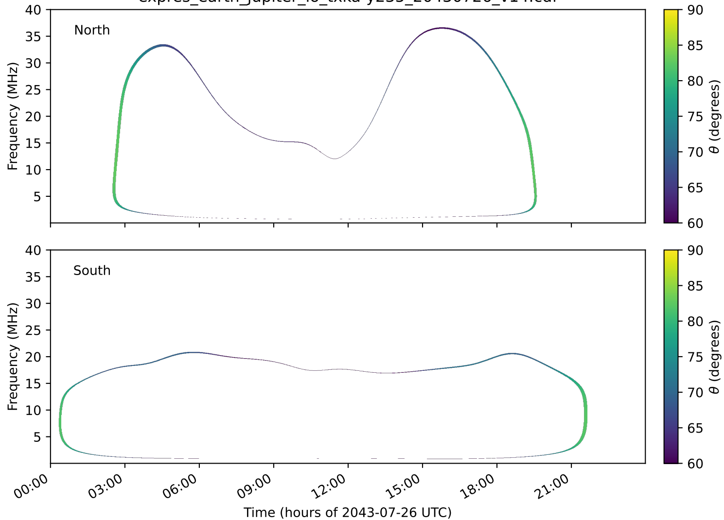
expres_earth_jupiter_io_txka-y235_20430726_v14.cdf
