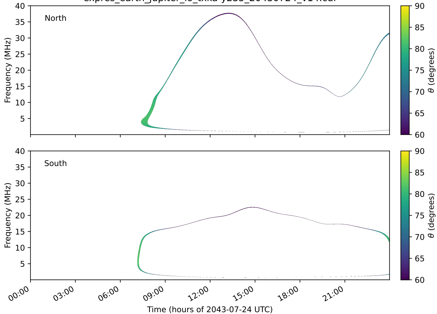
expres_earth_jupiter_io_txka-y235_20430724_v14.cdf
