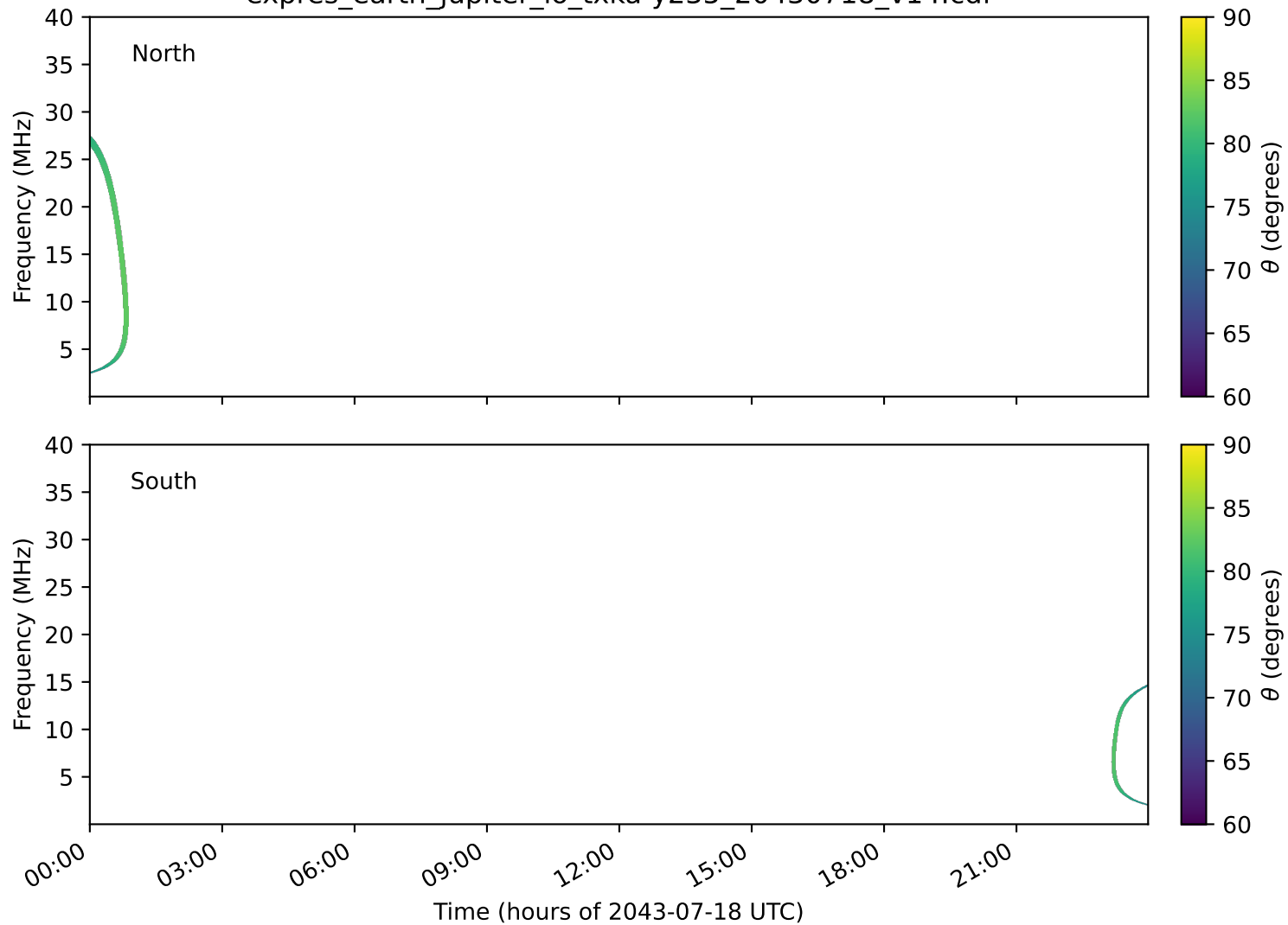
expres_earth_jupiter_io_txka-y235_20430718_v14.cdf
