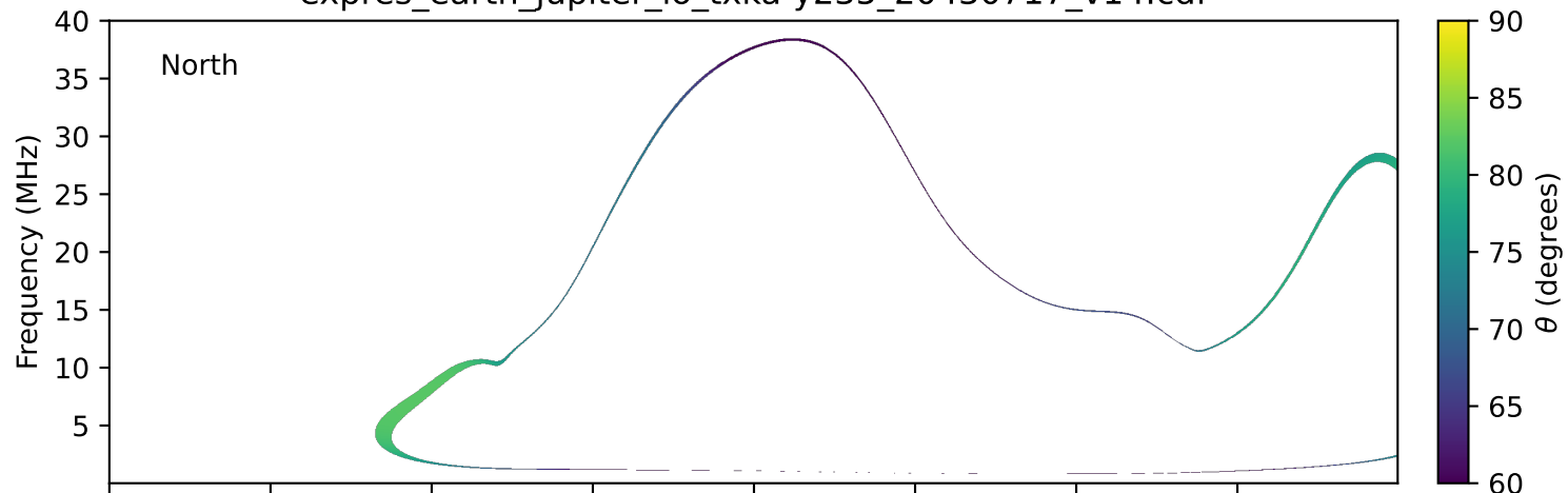
expres_earth_jupiter_io_txka-y235_20430717_v14.cdf
