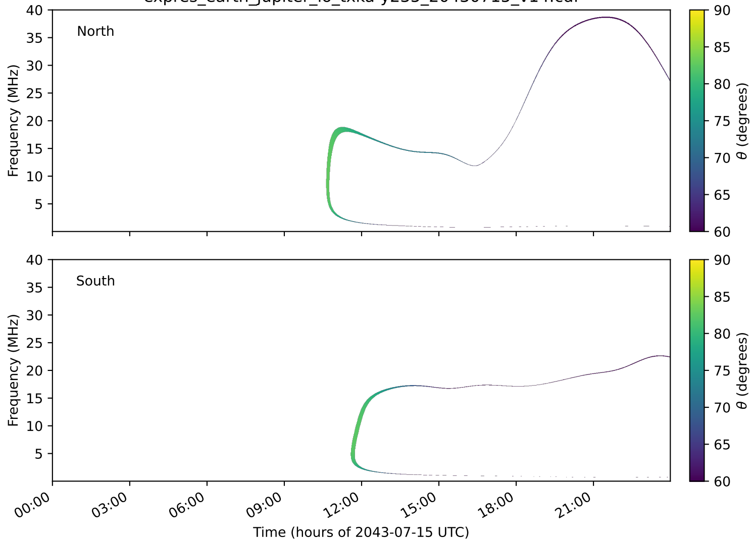
expres_earth_jupiter_io_txka-y235_20430715_v14.cdf
