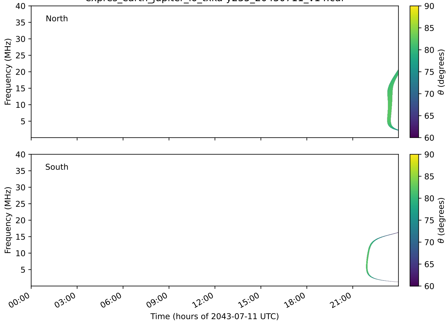
expres_earth_jupiter_io_txka-y235_20430711_v14.cdf
