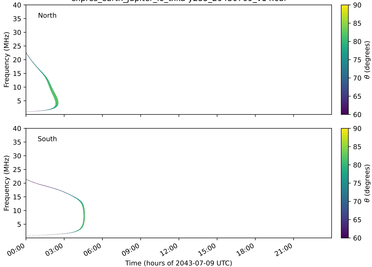
expres_earth_jupiter_io_txka-y235_20430709_v14.cdf
