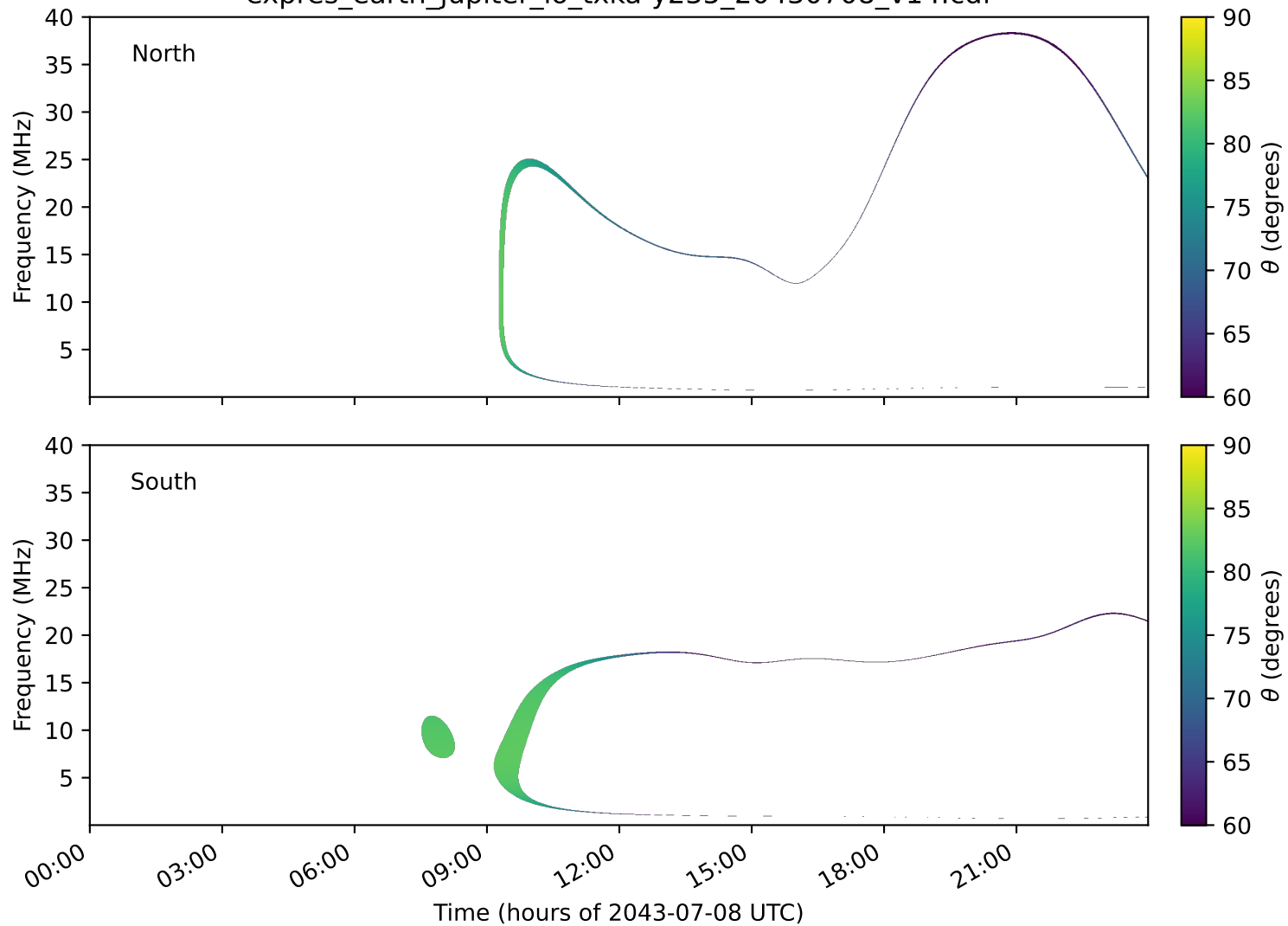
expres_earth_jupiter_io_txka-y235_20430708_v14.cdf
