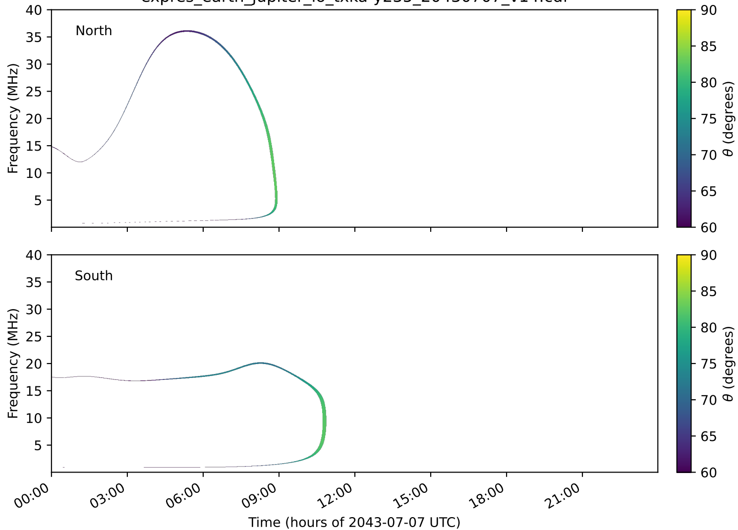
expres_earth_jupiter_io_txka-y235_20430707_v14.cdf
