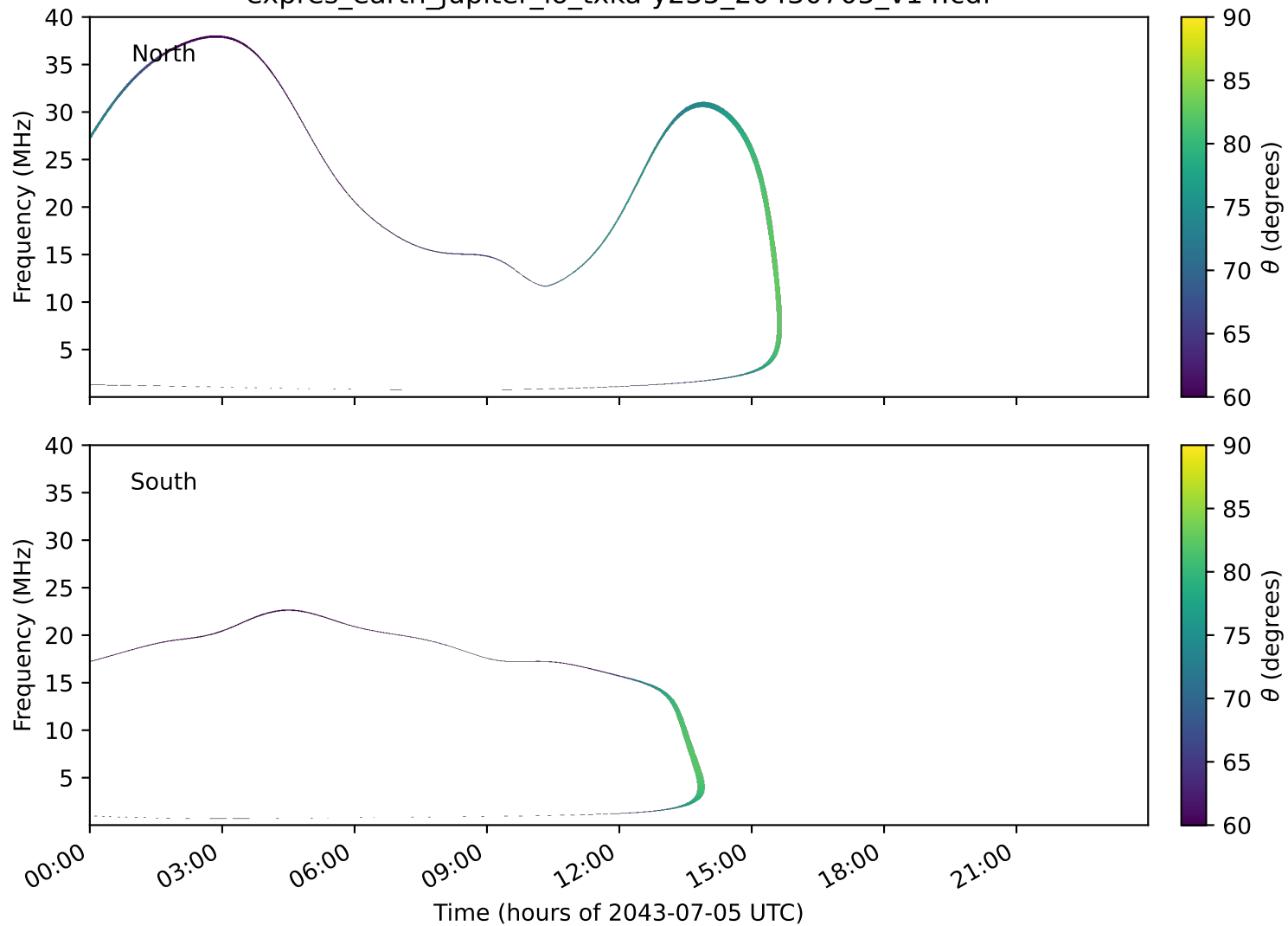
expres_earth_jupiter_io_txka-y235_20430705_v14.cdf
