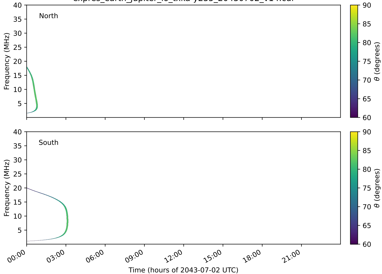
expres_earth_jupiter_io_txka-y235_20430702_v14.cdf
