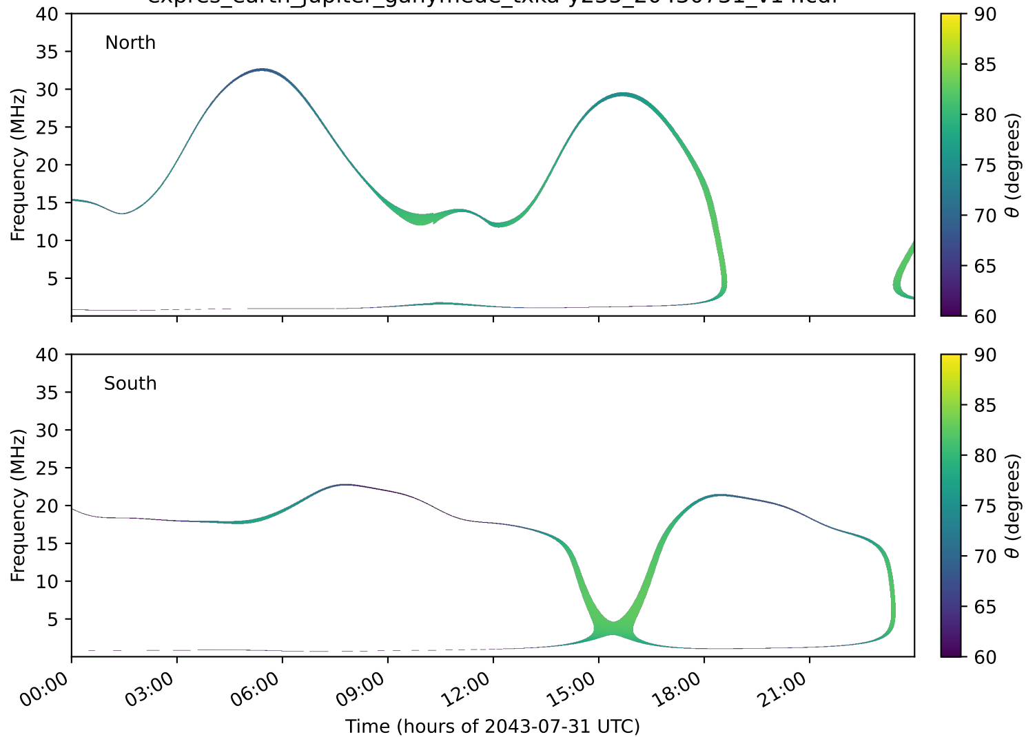
expres_earth_jupiter_ganymede_txka-y235_20430731_v14.cdf
