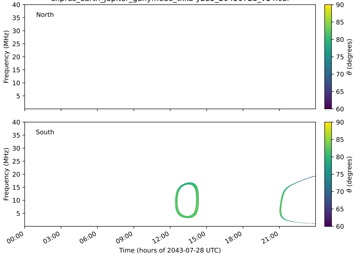
expres_earth_jupiter_ganymede_txka-y235_20430728_v14.cdf
