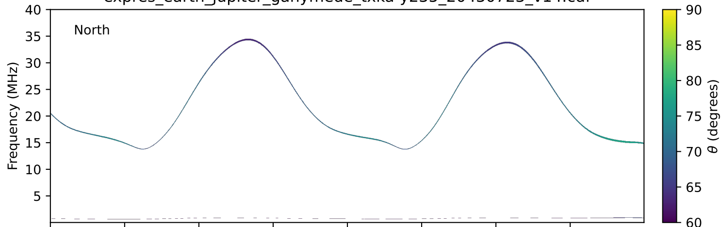
expres_earth_jupiter_ganymede_txka-y235_20430723_v14.cdf
