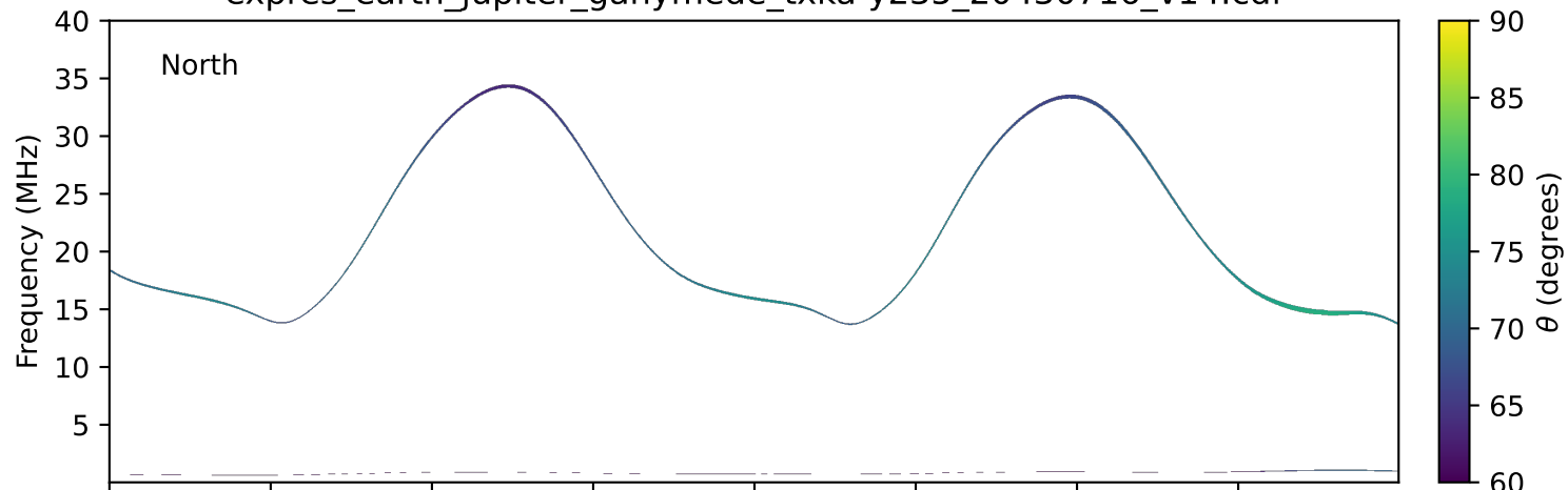
expres_earth_jupiter_ganymede_txka-y235_20430716_v14.cdf
