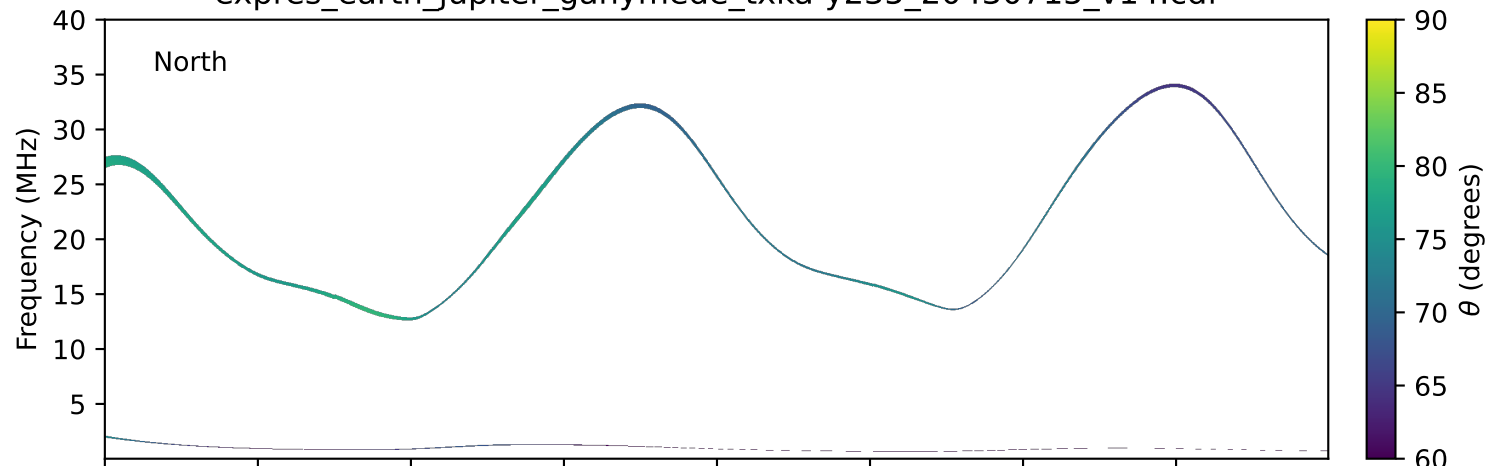
expres_earth_jupiter_ganymede_txka-y235_20430715_v14.cdf
