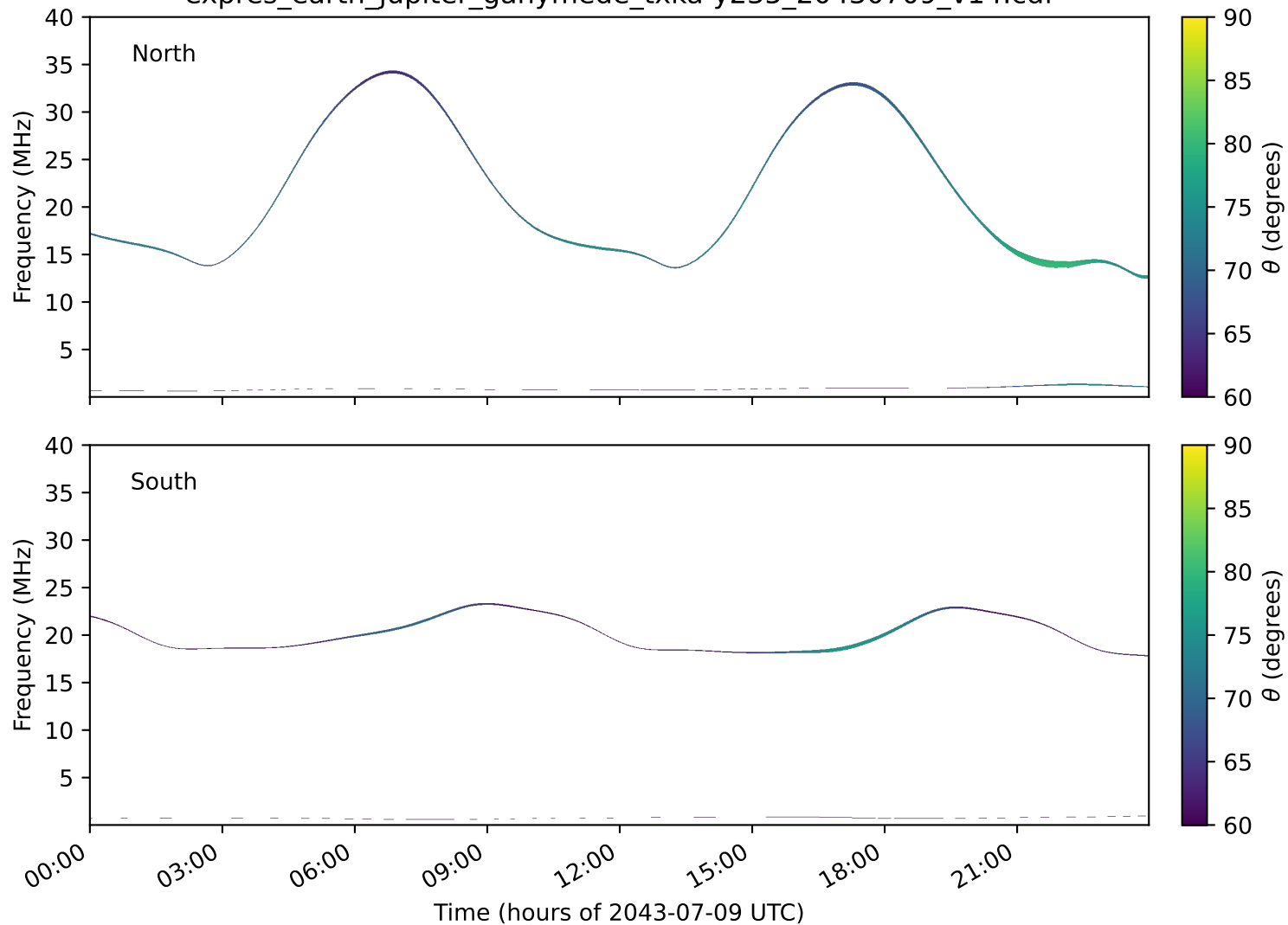
expres_earth_jupiter_ganymede_txka-y235_20430709_v14.cdf
