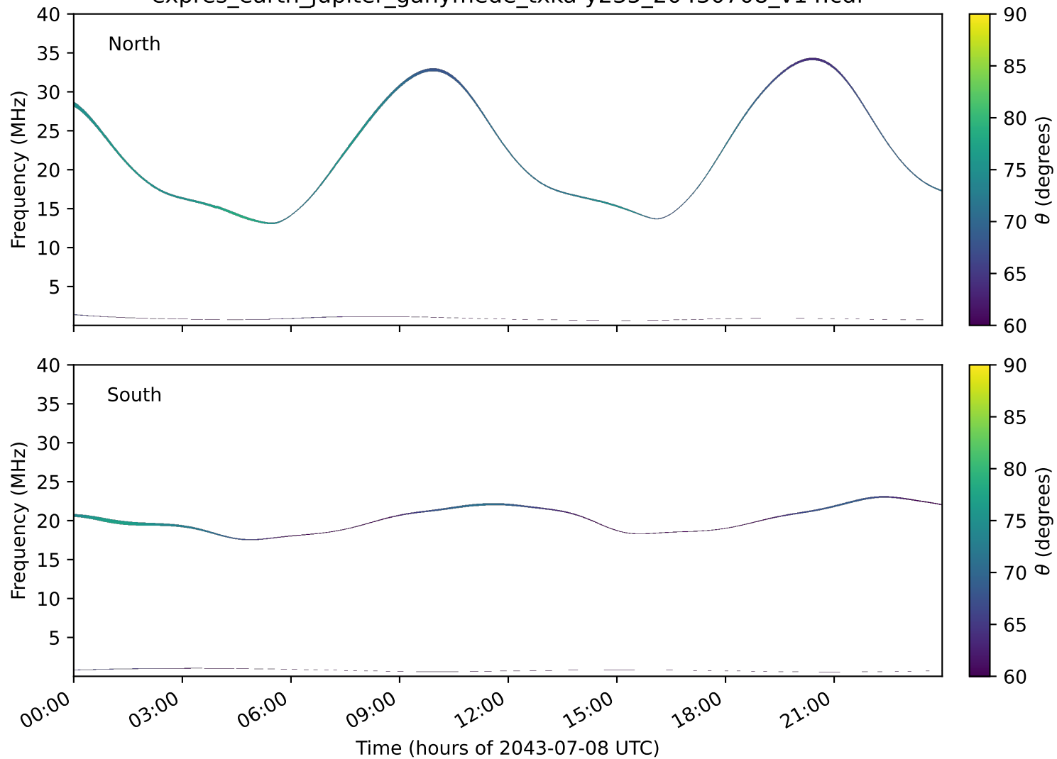
expres_earth_jupiter_ganymede_txka-y235_20430708_v14.cdf
