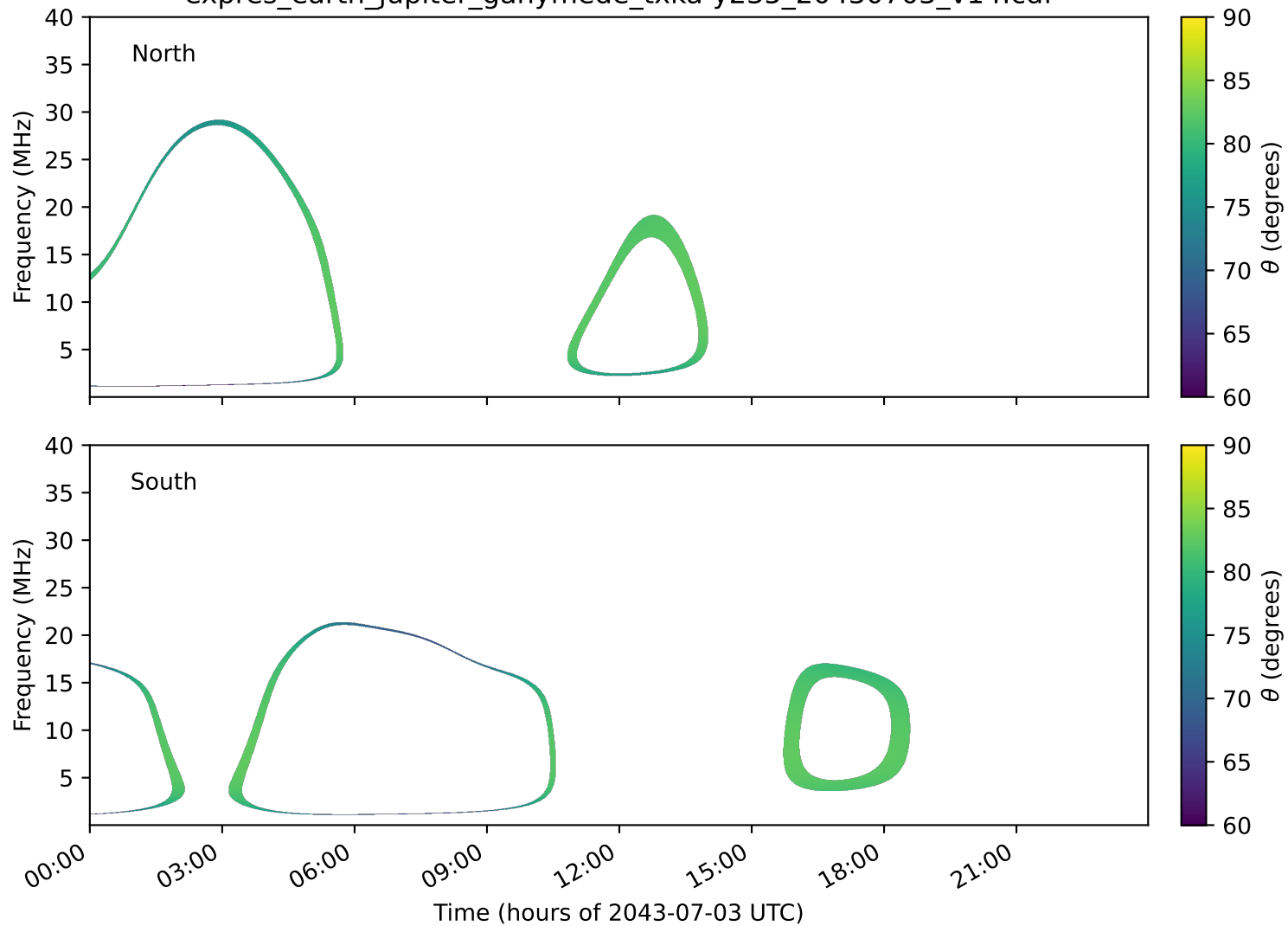
expres_earth_jupiter_ganymede_txka-y235_20430703_v14.cdf
