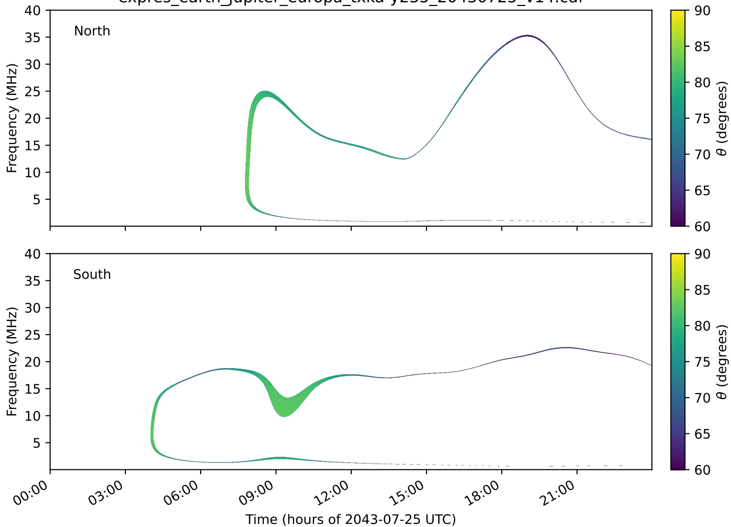
expres_earth_jupiter_europa_txka-y235_20430725_v14.cdf
