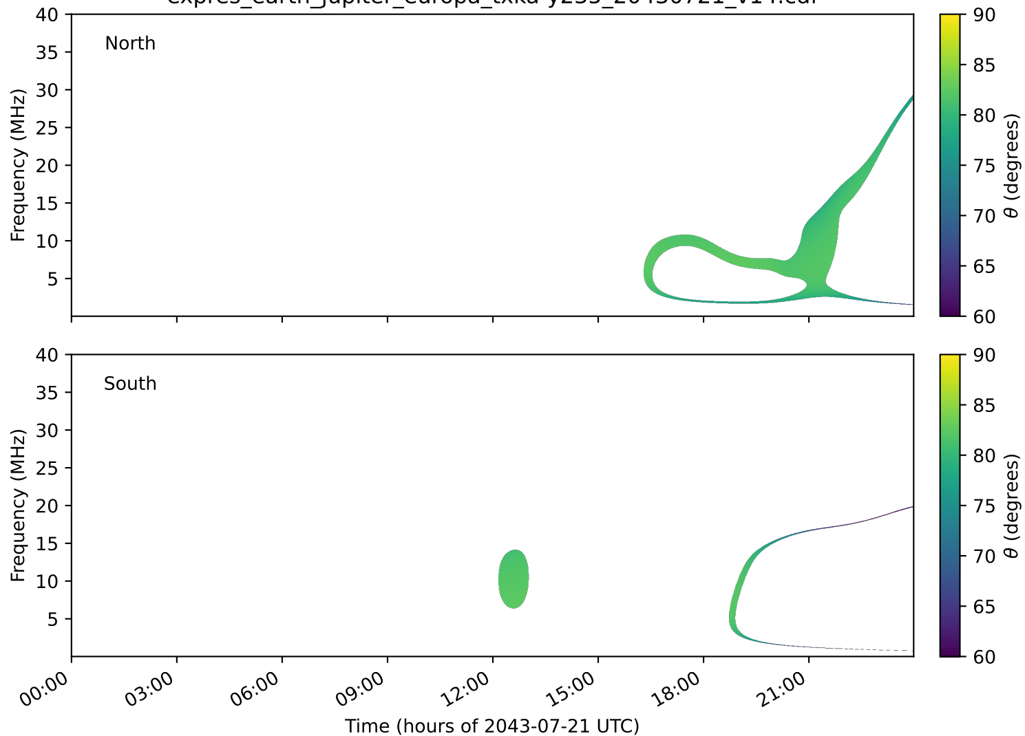
expres_earth_jupiter_europa_txka-y235_20430721_v14.cdf
