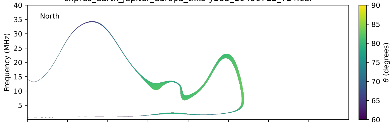
expres_earth_jupiter_europa_txka-y235_20430712_v14.cdf
