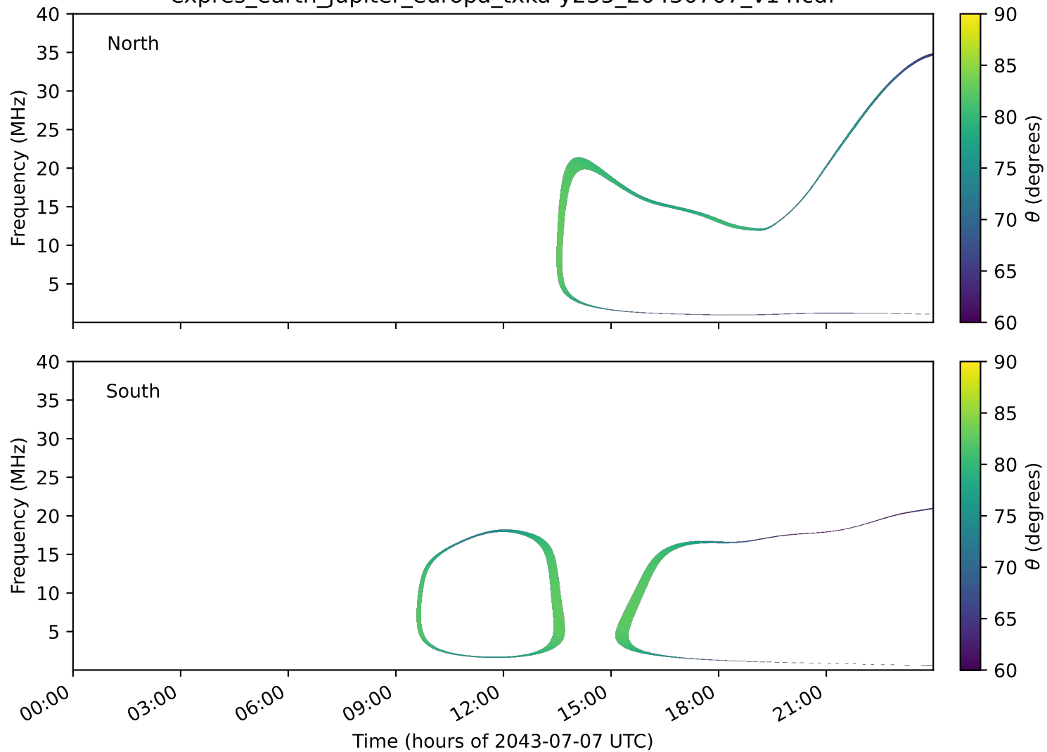
expres_earth_jupiter_europa_txka-y235_20430707_v14.cdf
