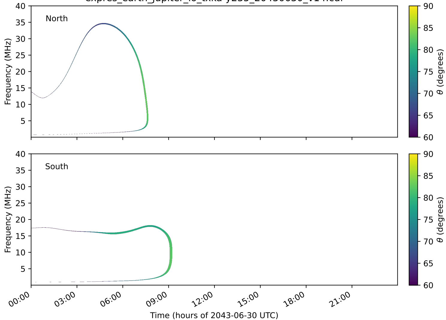
expres_earth_jupiter_io_txka-y235_20430630_v14.cdf
