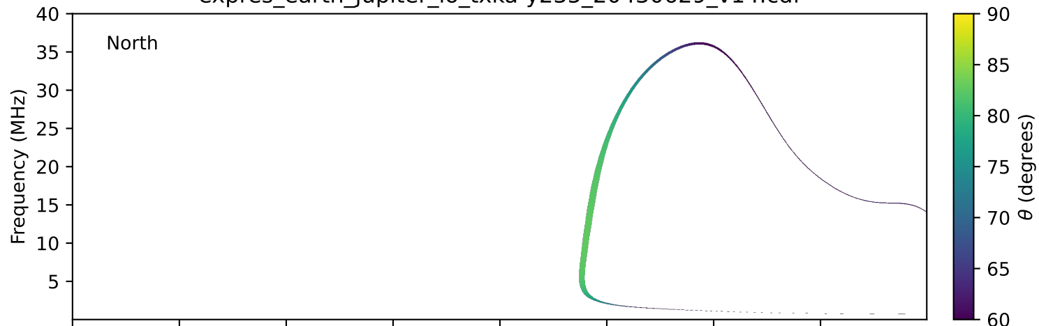
expres_earth_jupiter_io_txka-y235_20430629_v14.cdf
