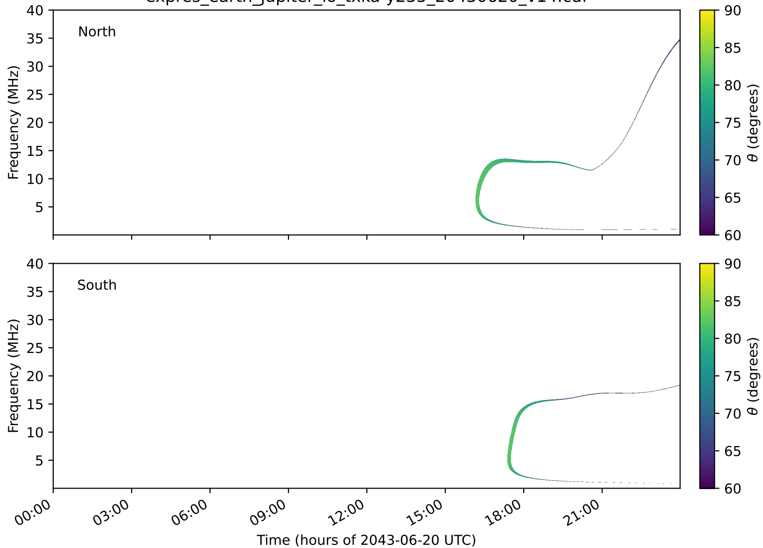
expres_earth_jupiter_io_txka-y235_20430620_v14.cdf
