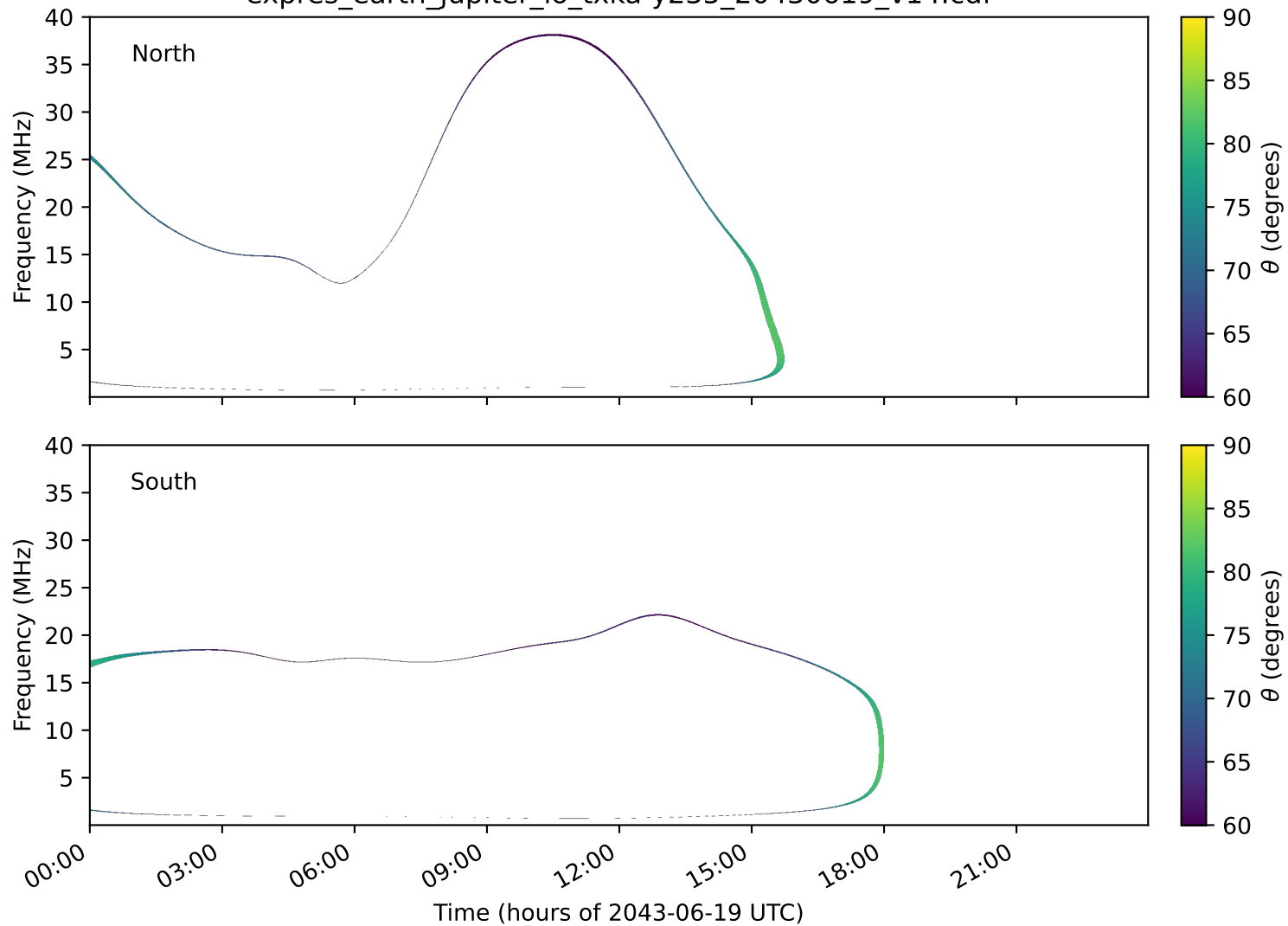
expres_earth_jupiter_io_txka-y235_20430619_v14.cdf
