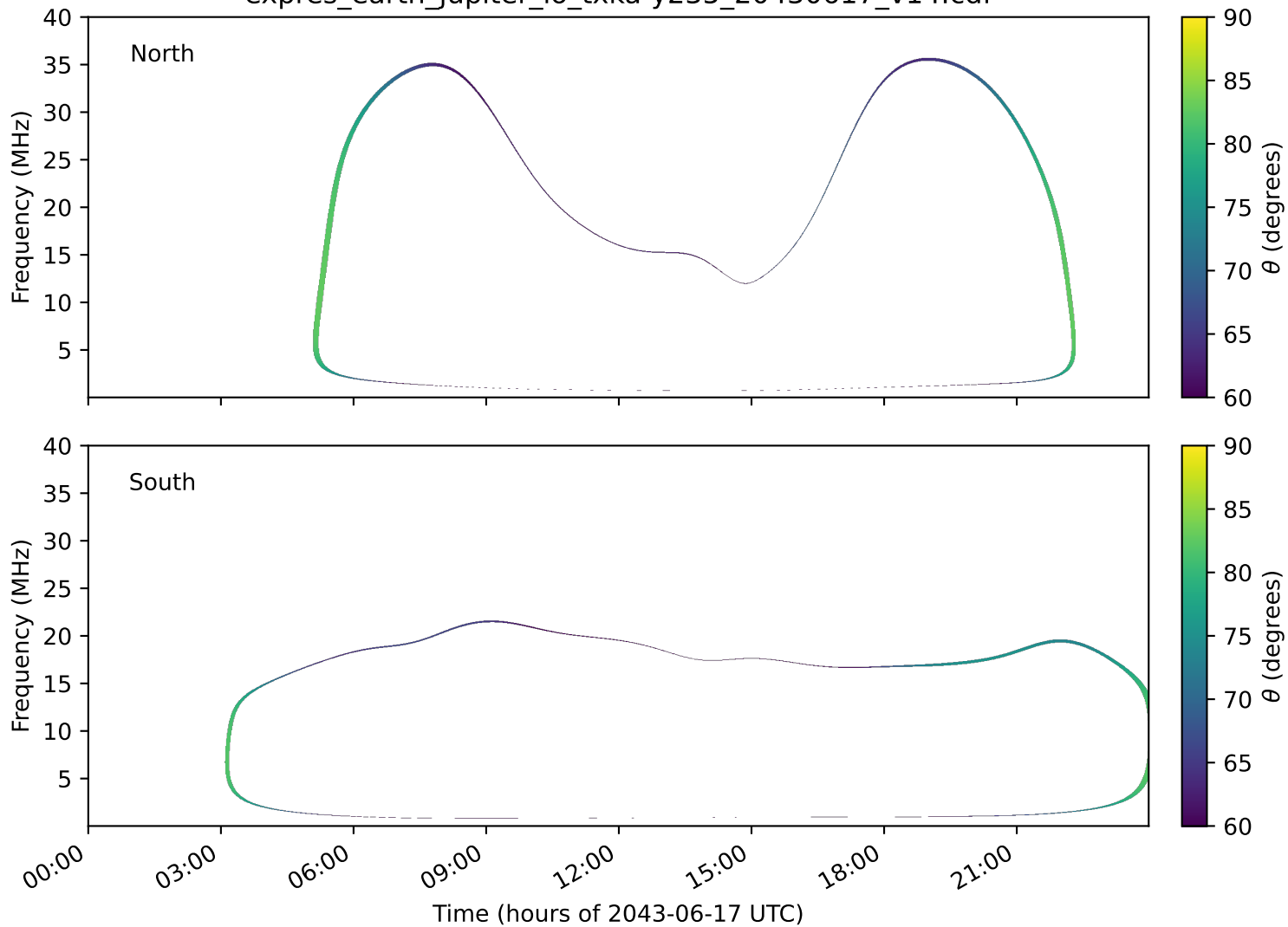
expres_earth_jupiter_io_txka-y235_20430617_v14.cdf
