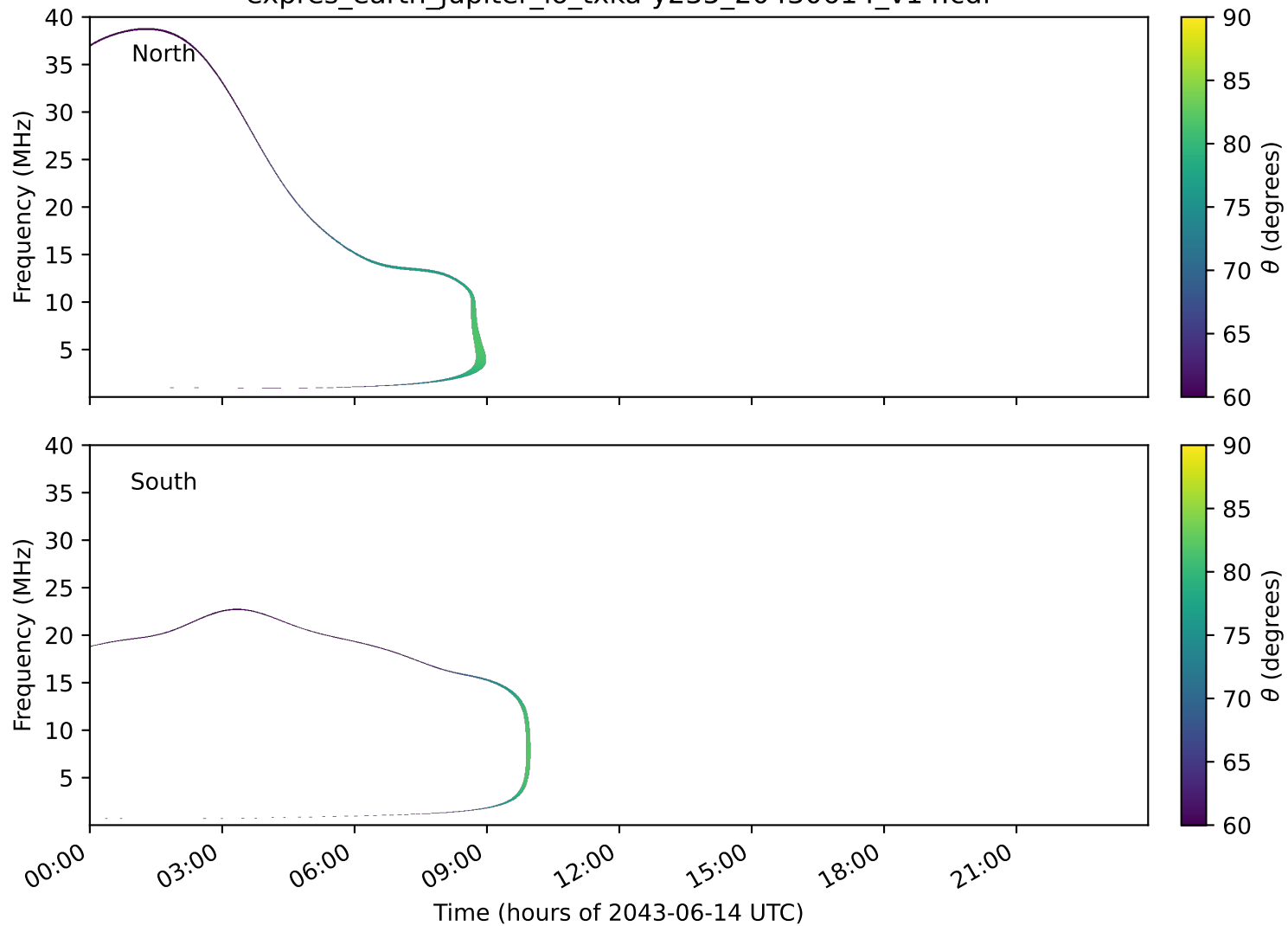
expres_earth_jupiter_io_txka-y235_20430614_v14.cdf
