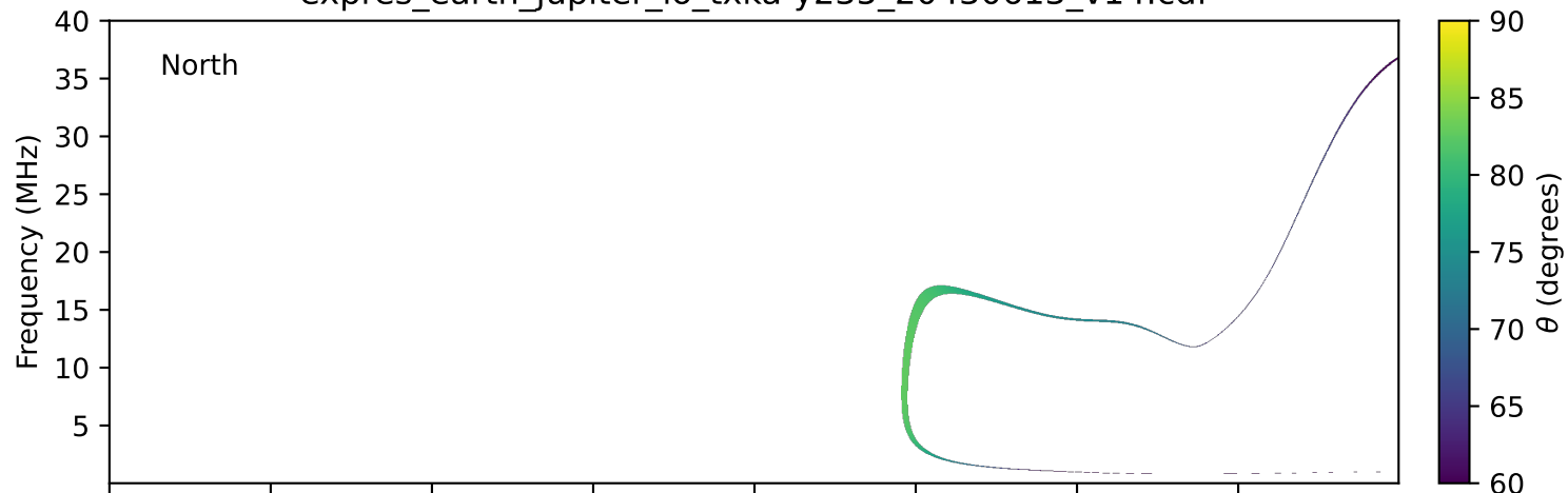
expres_earth_jupiter_io_txka-y235_20430613_v14.cdf
