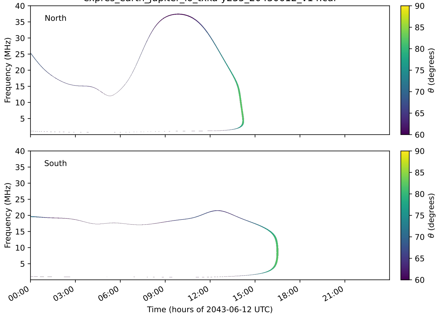
expres_earth_jupiter_io_txka-y235_20430612_v14.cdf
