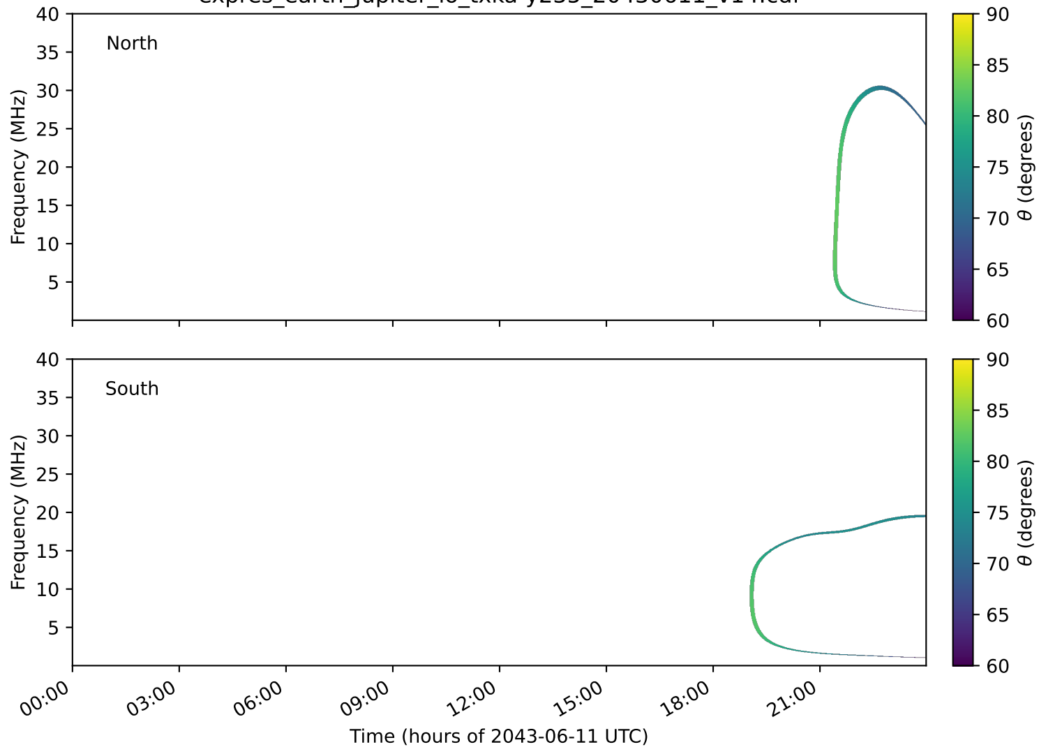
expres_earth_jupiter_io_txka-y235_20430611_v14.cdf
