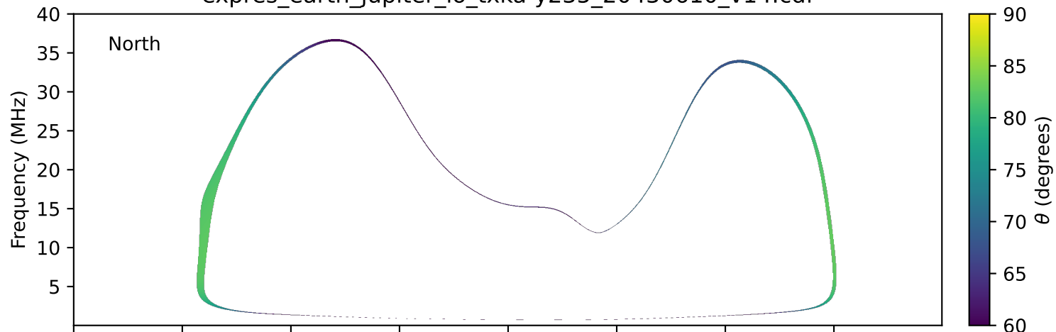
expres_earth_jupiter_io_txka-y235_20430610_v14.cdf
