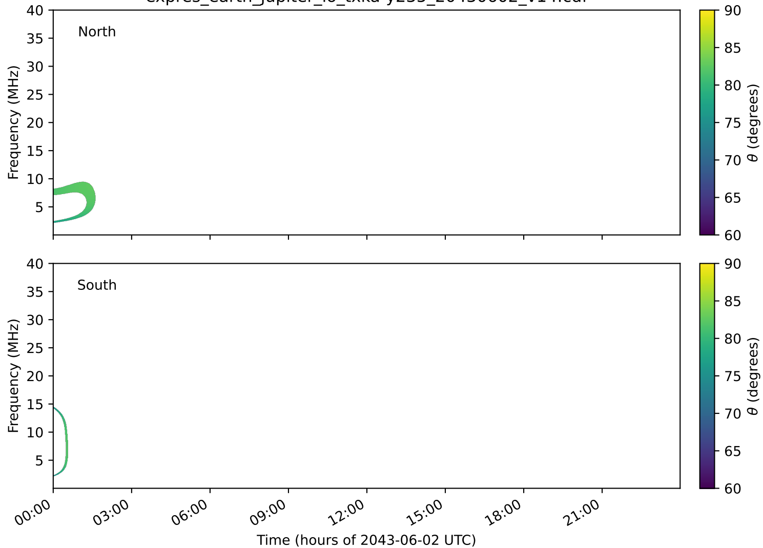
expres_earth_jupiter_io_txka-y235_20430602_v14.cdf
