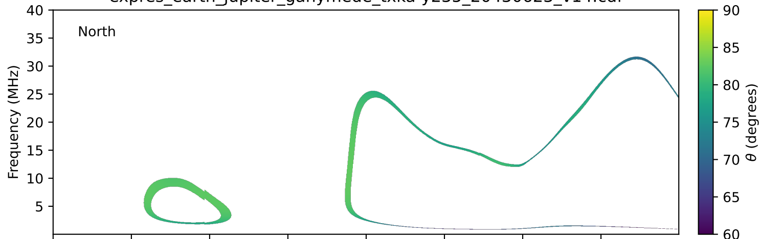
expres_earth_jupiter_ganymede_txka-y235_20430623_v14.cdf
