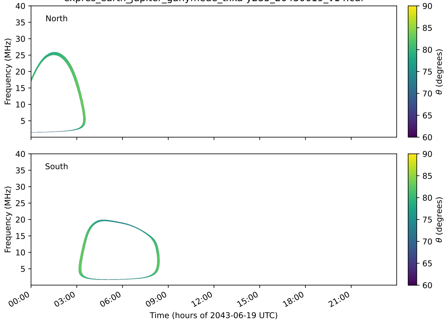
expres_earth_jupiter_ganymede_txka-y235_20430619_v14.cdf
