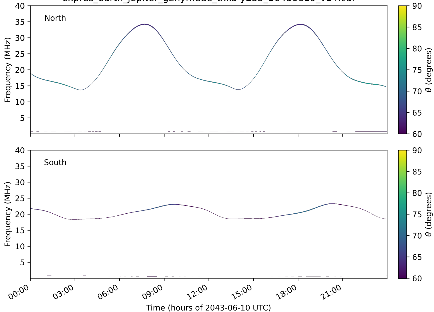
expres_earth_jupiter_ganymede_txka-y235_20430610_v14.cdf
