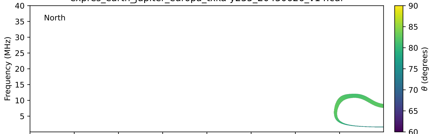
expres_earth_jupiter_europa_txka-y235_20430626_v14.cdf
